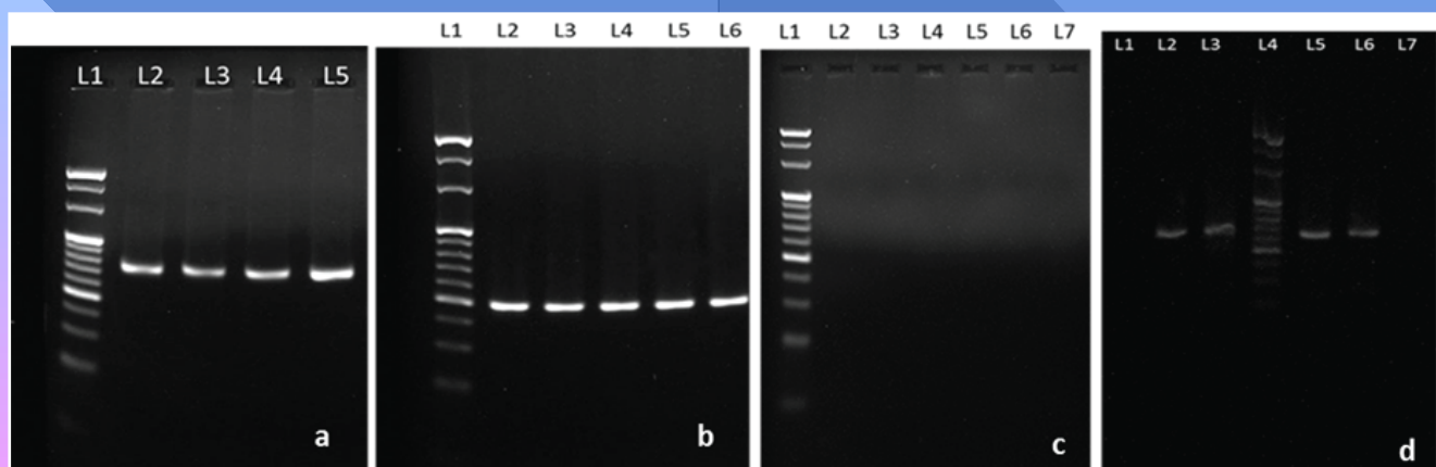
Fig.2: Gel profile of PCR product (a) stx1 , (b) stx2 , (c) no template control (NTC) for stx1 and stx2 gene of E. coli O 157 :H 7 and (d) Salmonella.
